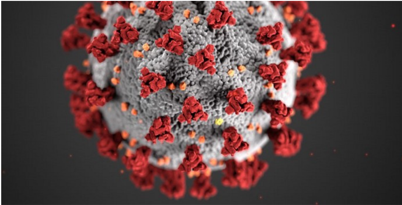
The spike proteins on the coronavirus's surface determine which animal it can infect. CDC.gov
